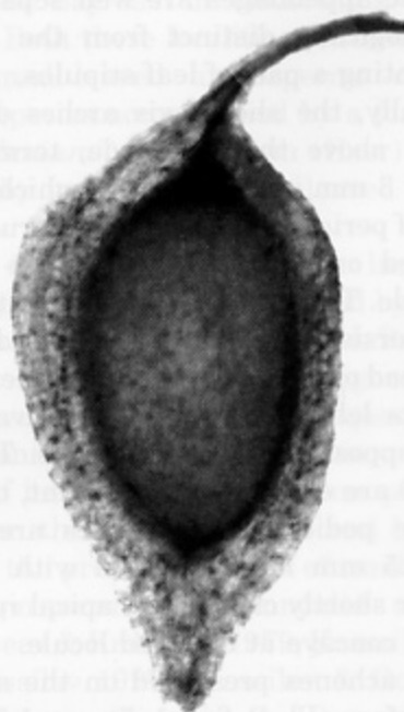
Fig. 2. Achene of extant Anemone coronaria L., extant on Mount Carmel, Israel, cleared to show the position of the seed for comparison with Pl. 2, figs 6, 7
