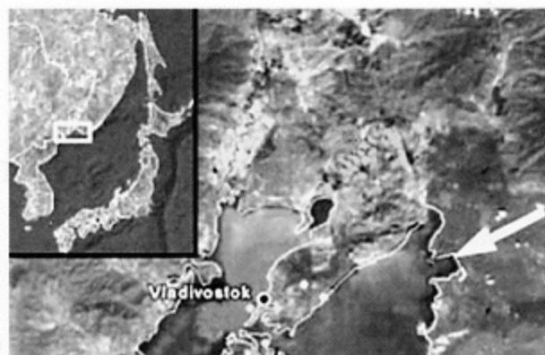
Fig. 1. Study area in the South Primorye. Arrow on the Ussuriysk Bay angiosperm locality
