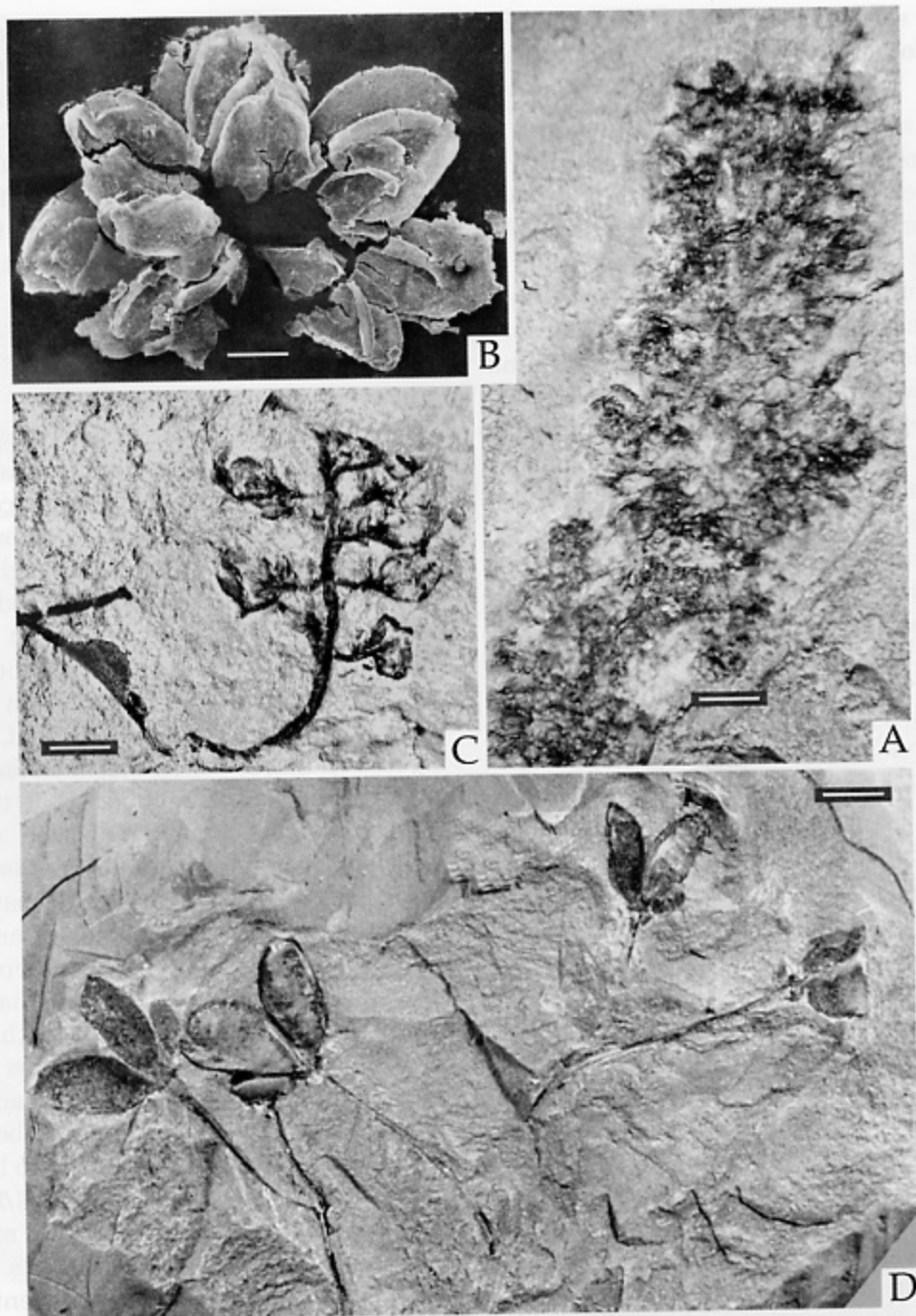
Fig. 4. Ranunculoid angiosperms from the Albian – Cenomanian of Siberia and Kazakhstan: A – Caspiocarpus paniculiger Krassilov & Vachrameev (Krassilov 1984); B – Callierypta chlamydea Krassilov & Golovneva (Krassilov & Golovneva 2004); C – Freyantha sibirica Krassilov & Golovneva (Krassilov & Golovneva 2001); D – Hyrcantha karatscheensis (Vachrameev) Krassilov (Krassilov et al. 1983). Scalebars: A – 1 mm; B – 0,3 mm; C, D – 3 mm
