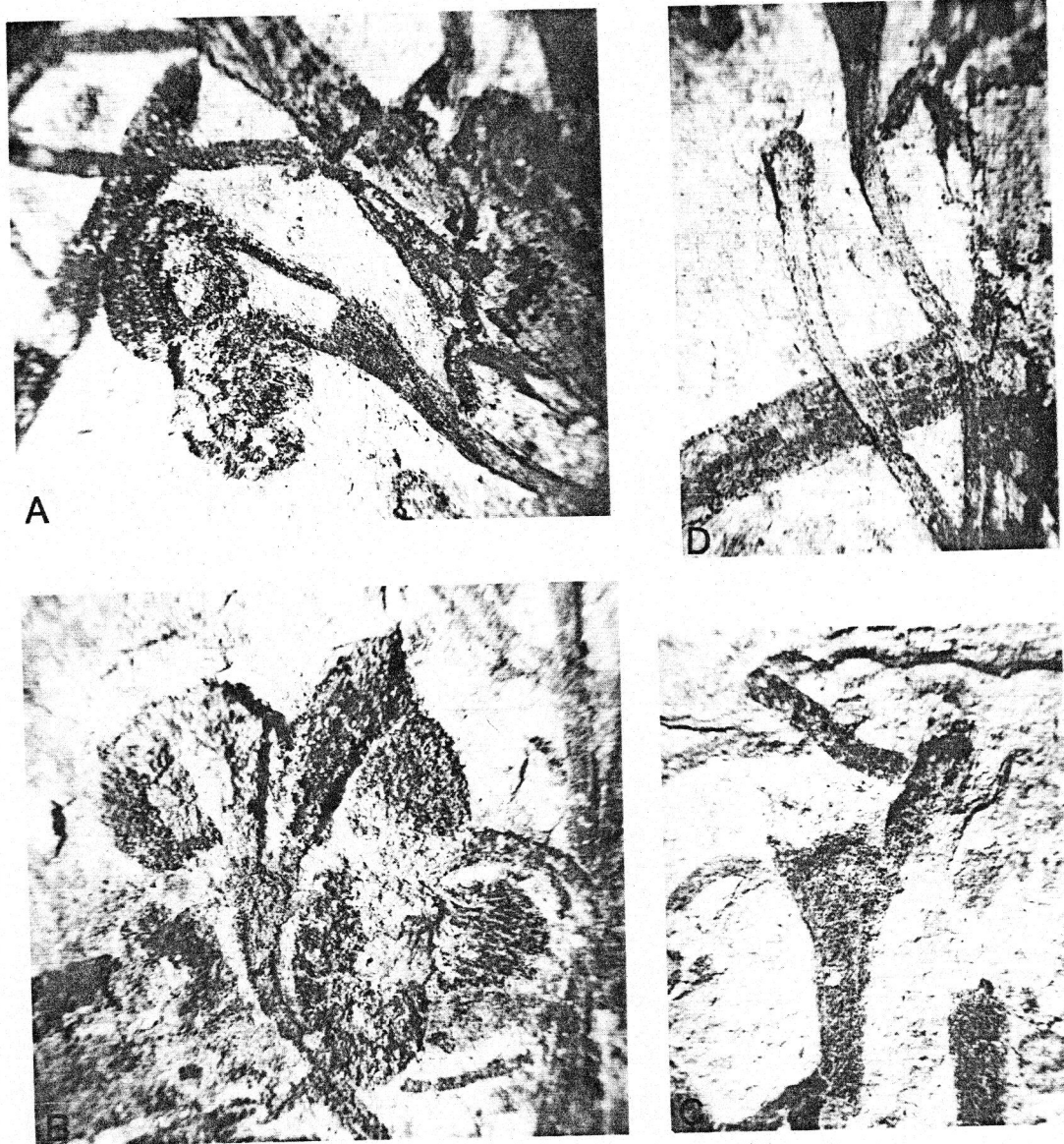
Fig. 3. Paracladia of Meeusella proteiclada sp. nov. □ A. With stalked sporangial heads, \times 10 . □ B–C. With subsessile heads, \times 12 . □ D. Sterile, \times 10 .
