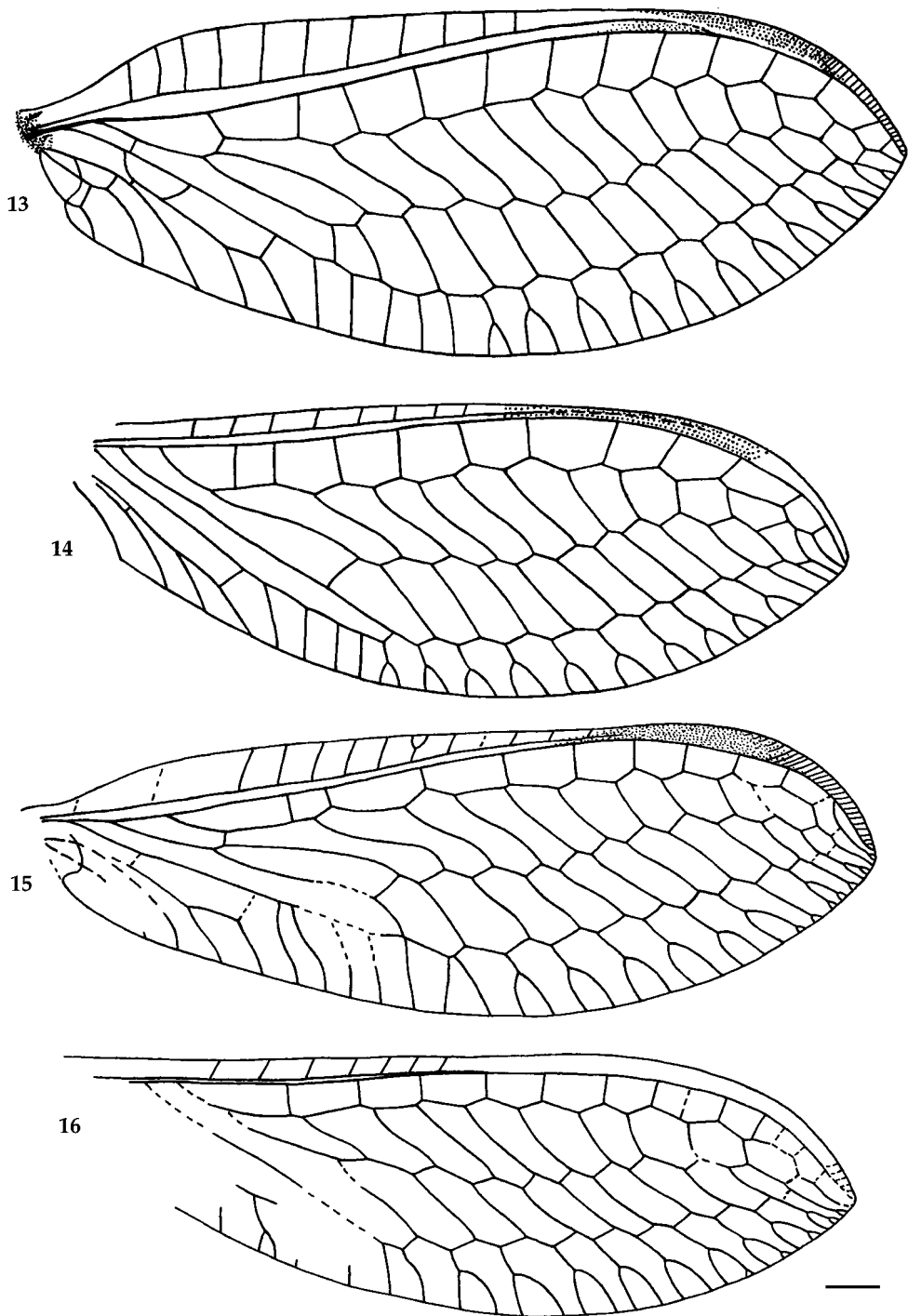
Figs 13-14. Mesypochrysa chrysopa , spec. nov. 13. Holotype, specimen N 3064/2432, forewing. 14. Paratype, specimen N 3064/2431, hindwing. Figs 15-16. Mesypochrysa curvimedia , spec. nov. 15. Holotype, specimen N 1989/44, forewing. 16. Same, hindwing. Scale: 1 mm.
