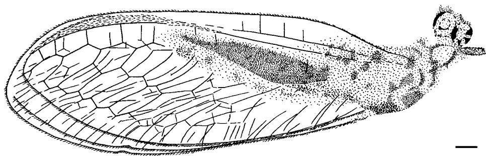
Fig. 19. Mesypochrysa spec. Specimen N 3064/2234. Scale: 1 mm.
