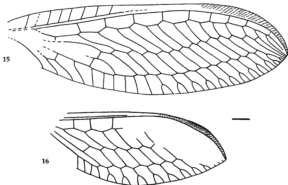
Fig. 17. Mesypochrysa angustialata , spec. nov. Holotype, specimen N 3064/2209, forewing.
