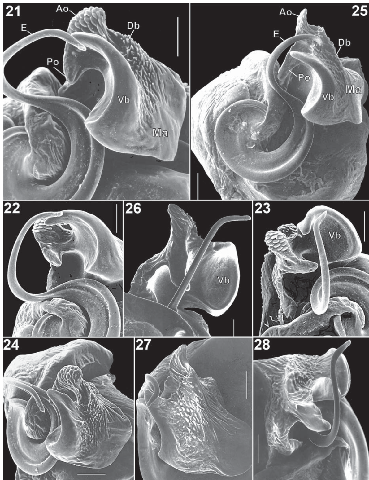
Figs 21–28. Embolic divisions of Synagelides agoriformis Strand, 1906 (21–24) and S. zhilcovaе Prószyński, 1979 (25–28): 21, 25 — ventral view; 22 — prolatero-ventral view; 26 — prolateral view; 23, 28 — anterior view; 24, 27 — antero-dorsal view. Scale bars: 0.1 mm. Abbreviations: Ao — anterior outgrowth; Db — dorsal branch, E — embolus, Ma — median apophysis, Po — posterior outgrowth, Vb — ventral branch.
