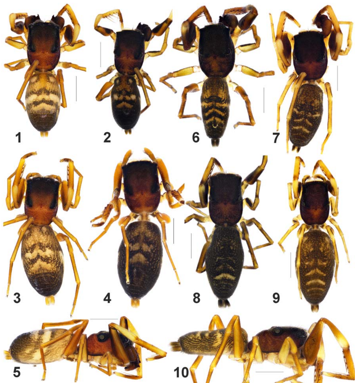
Figs 1–10. General appearance of Synagelides agoriformis Strand, 1906 (1–5) and S. zhilcova Prószyński, 1979 (6–10): 1, 2, 6, 7 — male, dorsal; 5, 10 — ditto, lateral view; 3, 4, 8, 9 — female, dorsal view. Specimens: 1, 3, 5 — from Liaoning Prov. (China); 2, 4, 6, 8–10 — from Maritime Territory (Russia); 7, 9 — from Shikotan Isl. (Russia). Scale bars: 1 mm.
