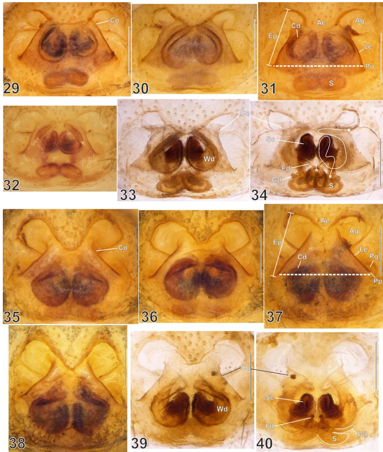
Figs 29–40. Epigyne of Synagelides agoriformis Strand, 1906 (29–34) and S. zhilcova Prószyński, 1979 (35–40): 29–32, 35–38 — intact epigyne, ventral view; 33, 39 — macerated epigyne, ventral view; 34, 40 — macerated vulva, dorsal view. Scale bars: 0.2 mm. Abbreviations: Ae — anterior edge of epigyne, Ag — anterior groove of epigyne pocket, Cd — copulatory duct, Co — copulatory opening, Ep — pocket of epigyne, Fd — fertilization duct, Gd — glandular duct, Le — lateral edge of epigyne, Pg — posterior groove of epigyne pocket, Pp — posterior edge of epigyne pocket, S — spermathecae, Sc — sclerotized curve of copulatory ducts, Wd — widened part of copulatory duct.
