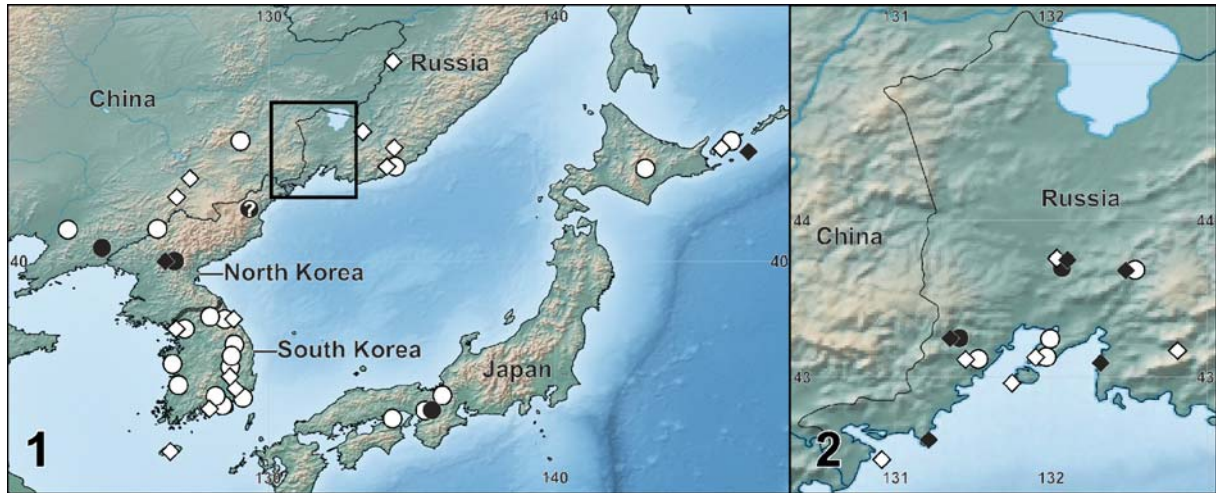
Maps 1, 2. Collecting localities of Synagelides agoriformis Strand, 1906 (circle) and S. zhilcova Prószyński, 1979 (diamond). Black symbols refer to the studied material, white symbols refer to the literature-derived data. Question mark in circle designates an unclear locality. Some symbols on Map 1 could refer to more than one closely situated localities. The frame of Map 1 refers to the content of Map 2.
