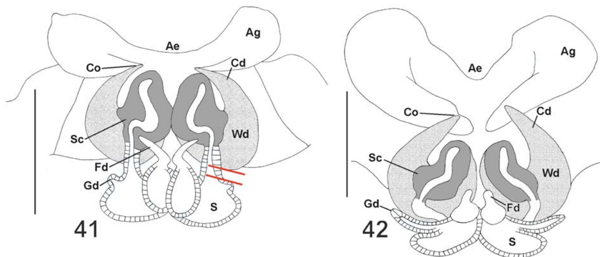
Figs 41–42. Vulva of Synagelides agoriformis Strand, 1906 (41) and S. zhilcova Prószyński, 1979 (42). Scale bars: 0.2 mm. Abbreviations: Ae — anterior edge of epigyne; Ag — anterior groove of epigyne pocket, Cd — copulatory duct, Co — copulatory opening, Fd — fertilization duct, Gd — glandular duct, S — spermathecae, Sc — sclerotized curve of copulatory ducts, Wd — widened part of copulatory duct.
