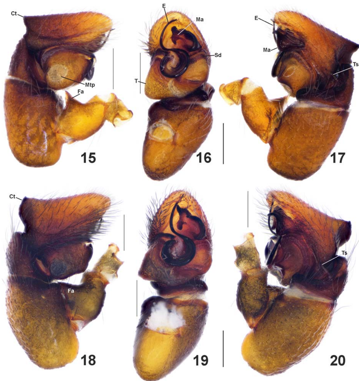
Figs 15–20. Male palps of Synagelides agoriformis Strand, 1906 (15–17) and S. zhilcovaе Prószyński, 1979 (18–20): 15, 18 — prolateral view; 16, 19 — ventral view; 17, 20 — retrolateral view. Scale bars: 0.25 mm. Abbreviations: Ct — prolateral cymbium tooth, E — embolus, Fa — prolateral femoral apophysis, Ma — median apophysis, Mtp — membranous tegular peak, Sd — sperm duct, T — tegulum, Ts — tibial spine.
