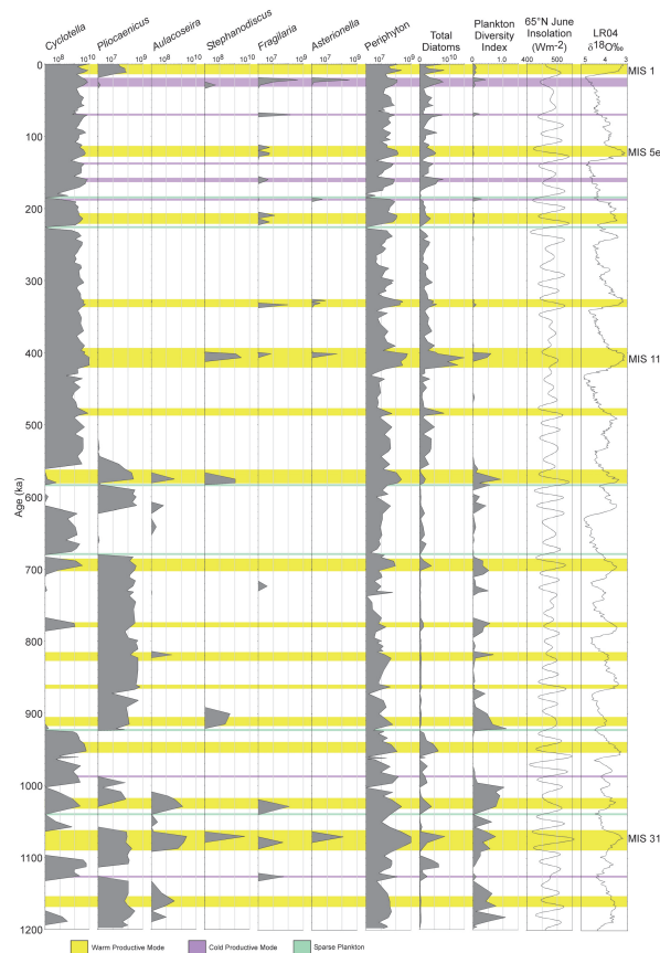
Fig. 2. Concentration (valves \text{g}^{-1} ) of planktonic species, total periphyton, total diatoms, and plankton diversity (Shannon Index) from 0–1.2 Ma. Exceptional events are indicated by colored intervals. Diatom concentrations, except total diatoms, are plotted on a log scale with range appropriate to the observed variation in the core record. For comparison, the marine isotope stack (Lisiecki and Raymo, 2005) and 65^\circ \text{N} June insolation (Laskar et al., 2004) are also plotted.
