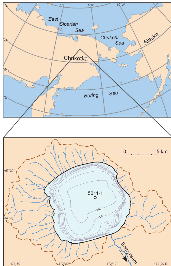
Fig. 1. Location map of Lake El'gygytyn and its catchment. Bathymetry (20-m contour interval) and stream network are modified from Nolan and Brigham-Grette (2007).
