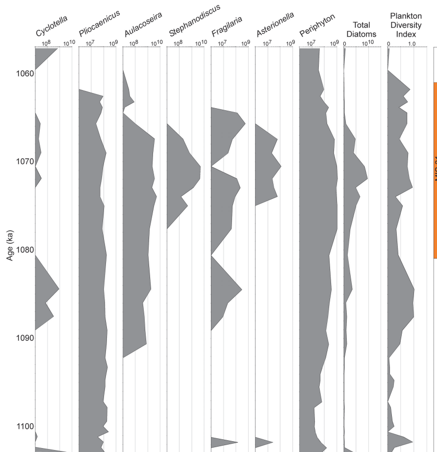
Fig. 6. Concentration (valves \text{g}^{-1} ) of planktonic species, total periphyton, total diatoms, and plankton diversity (Shannon Index) from 1057–1103 ka. Peak MIS 31 warmth indicated by other proxies (Melles et al., 2012) is also shown.
