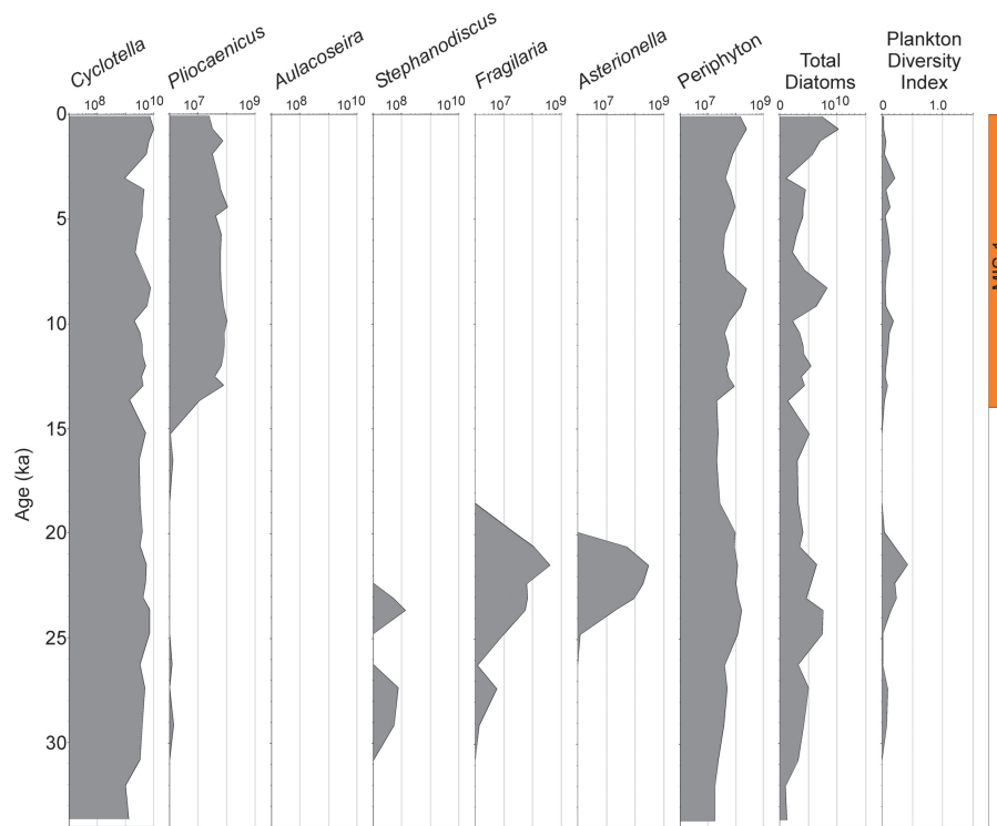
Fig. 3. Concentration (valves \text{g}^{-1} ) of planktonic species, total periphyton, total diatoms, and plankton diversity (Shannon Index) from 0–34 ka. Peak MIS 1 warmth indicated by other proxies (Melles et al., 2012) is also shown.
