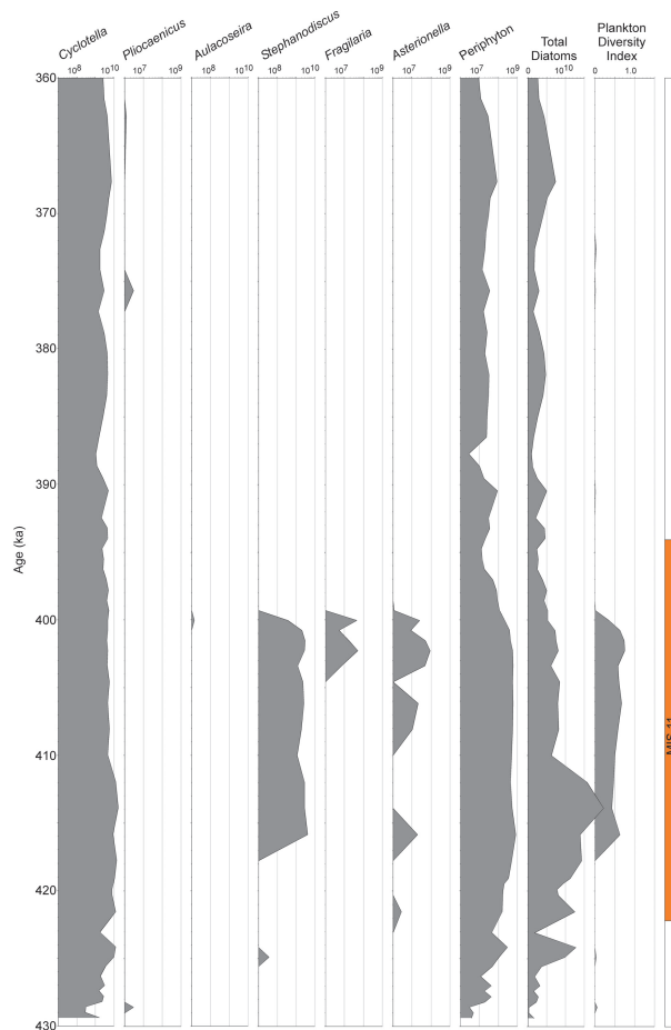
Fig. 5. Concentration (valves \text{g}^{-1} ) of planktonic species, total periphyton, total diatoms, and plankton diversity (Shannon Index) from 360–430 ka. Peak MIS 11 warmth indicated by other proxies (Melles et al., 2012) is also shown.
