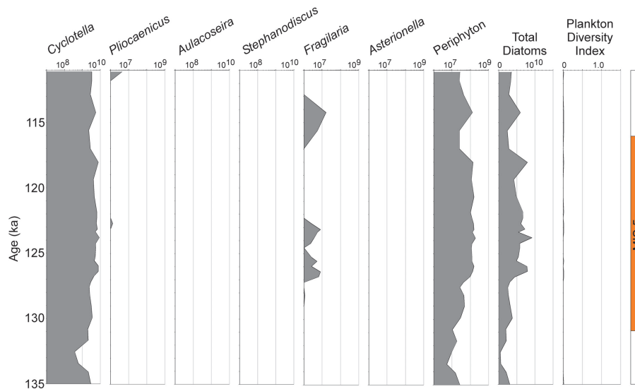
Fig. 4. Concentration (valves \text{g}^{-1} ) of planktonic species, total periphyton, total diatoms, and plankton diversity (Shannon Index) from 111–135 ka. Peak MIS 5e warmth indicated by other proxies (Melles et al., 2012) is also shown.
