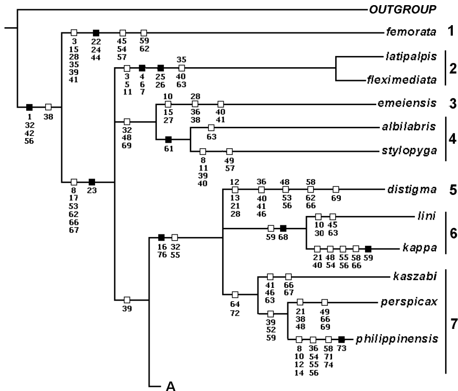
Fig. 1. The Adams consensus tree (length of 328 steps, CI – 0.3865, HI – 0.6135, RI – 0.6311, RC – 0.2439) of 1512 maximum parsimony trees resulting from cladistic analysis by PAUP (4.0b8) with indication of apomorphies (■) occurring only once on the tree; homoplasies (□). Outgroup – Diastatidae + Campichoetidae + Curtonotidae; tribe Gitonini (1-7): 1 – Parastegana ; 2 – Pseudostegana ; 3 – Paraleucophenga ; 4 – Amiota s. str.; 5 – Gitona ; 6 – Amiota (subgenera Apsiphortica and Phortica ); 7 – Cacoxenus . Tribe Steganini (8-11): subtribe Leucophengina (8): 8 – Leucophenga ; subtribe Steganina (9-12): 9-12 – Stegana (subgenera Anastega – 9; Stegana – 10; Oxyphortica – 12).
